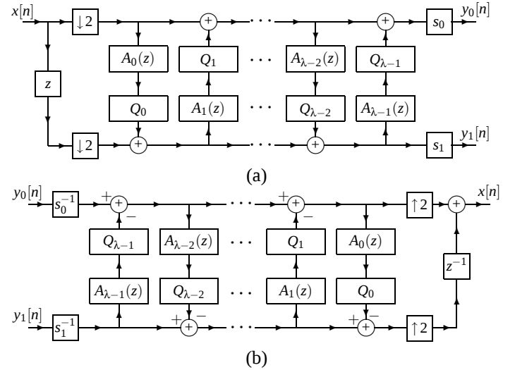
Fig. 6. Lifting realization of a 1-D 2-channel PR UMDFB. (a) Analysis side. (b) Synthesis side.
