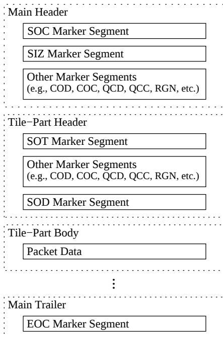
Fig. 14. Code stream structure.
