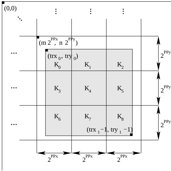
Fig. 11. Partitioning of a resolution into precincts.
