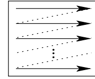
Fig. 12. Code block scan order within a precinct.
